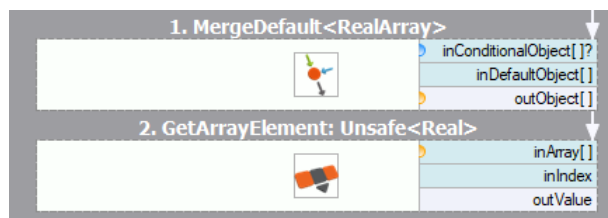
An example of two generic filters in the Program Editor: MergeDefault instantiated for replacing Nils in arrays of real numbers and GetArrayElement instantiated for getting a single element from them. Please note that the type parameter specified is different.
